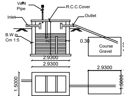
SEPTIC TANK & D-TRENCH DETAILS
