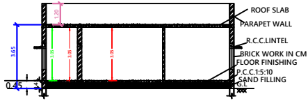
SECTION ON SS
