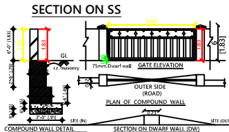
SECTION ON SS
