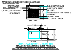
DETAILS OF COLLECTION SUMP FOR RAIN WATER
