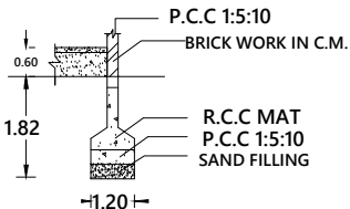
FOUNDATION DETAILS
