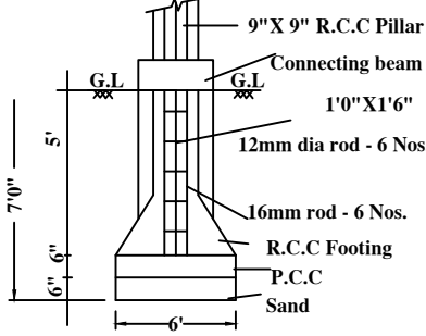
COLOUMN FOUNDATION DETAILS
