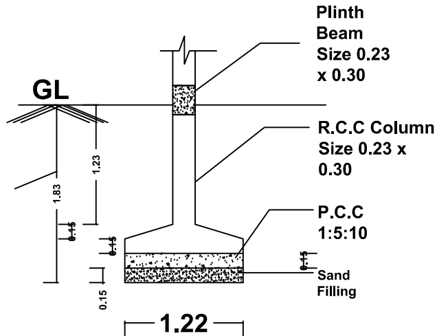
FOUNDATION DETAILS
