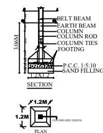
FOUNDATION DETAILS
