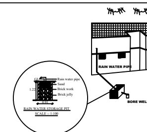
RAIN WATER STORAGE SYSTEM
