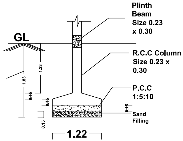
FOUNDATION DETAILS
