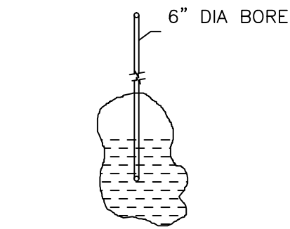
BORE WELL
