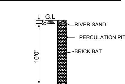
PERCULATION PIT
