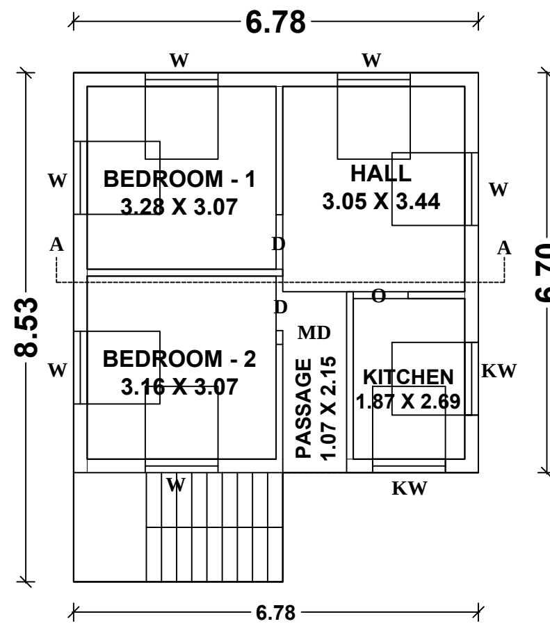
FLOOR- GROUND
