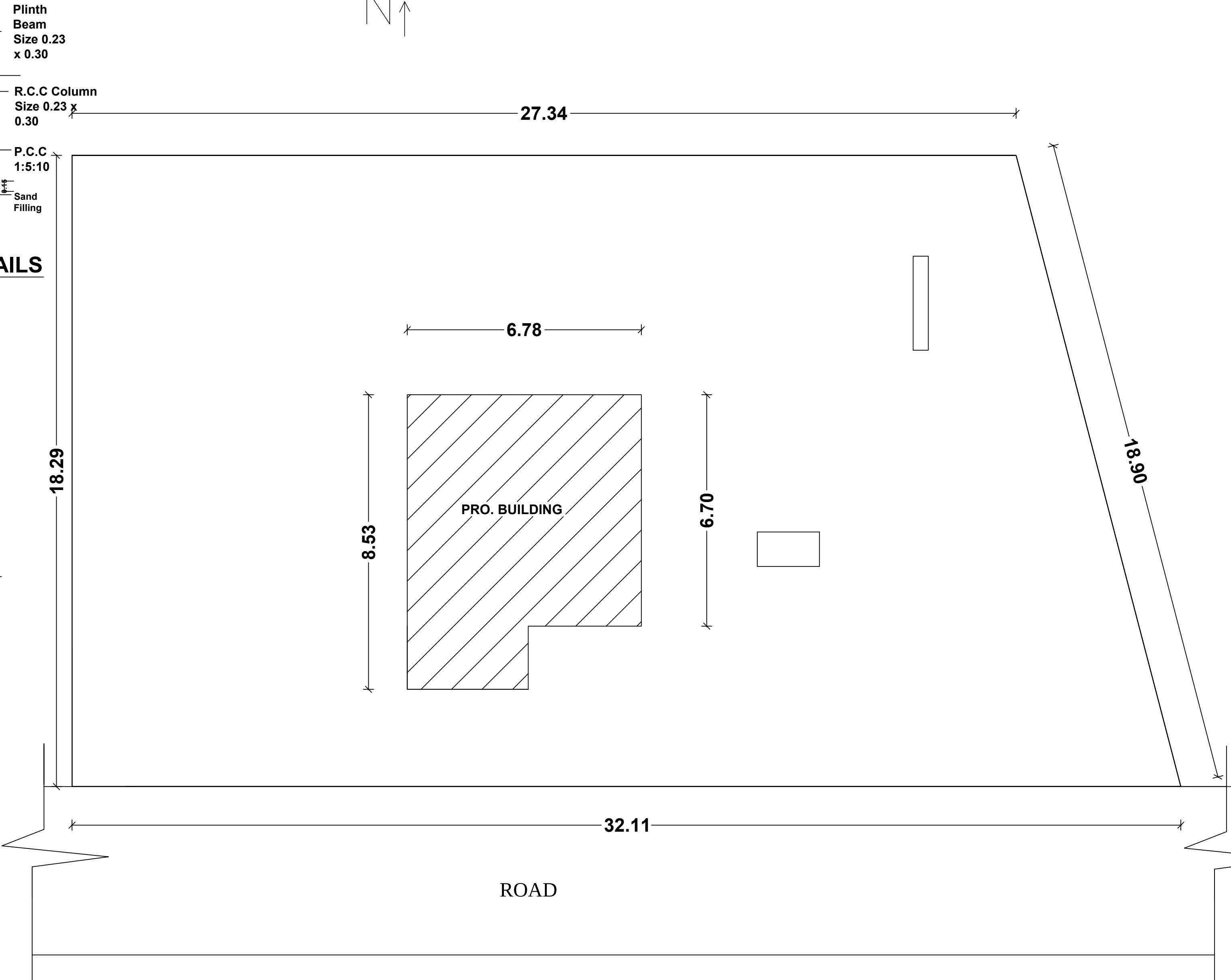
SITE PLAN
