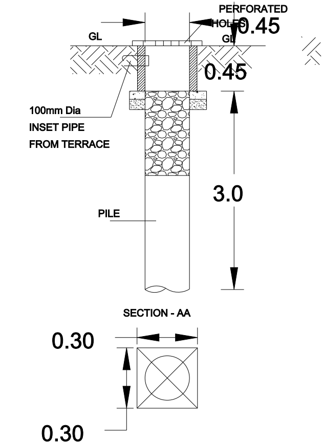
RWH TYPICAL DETAIL
