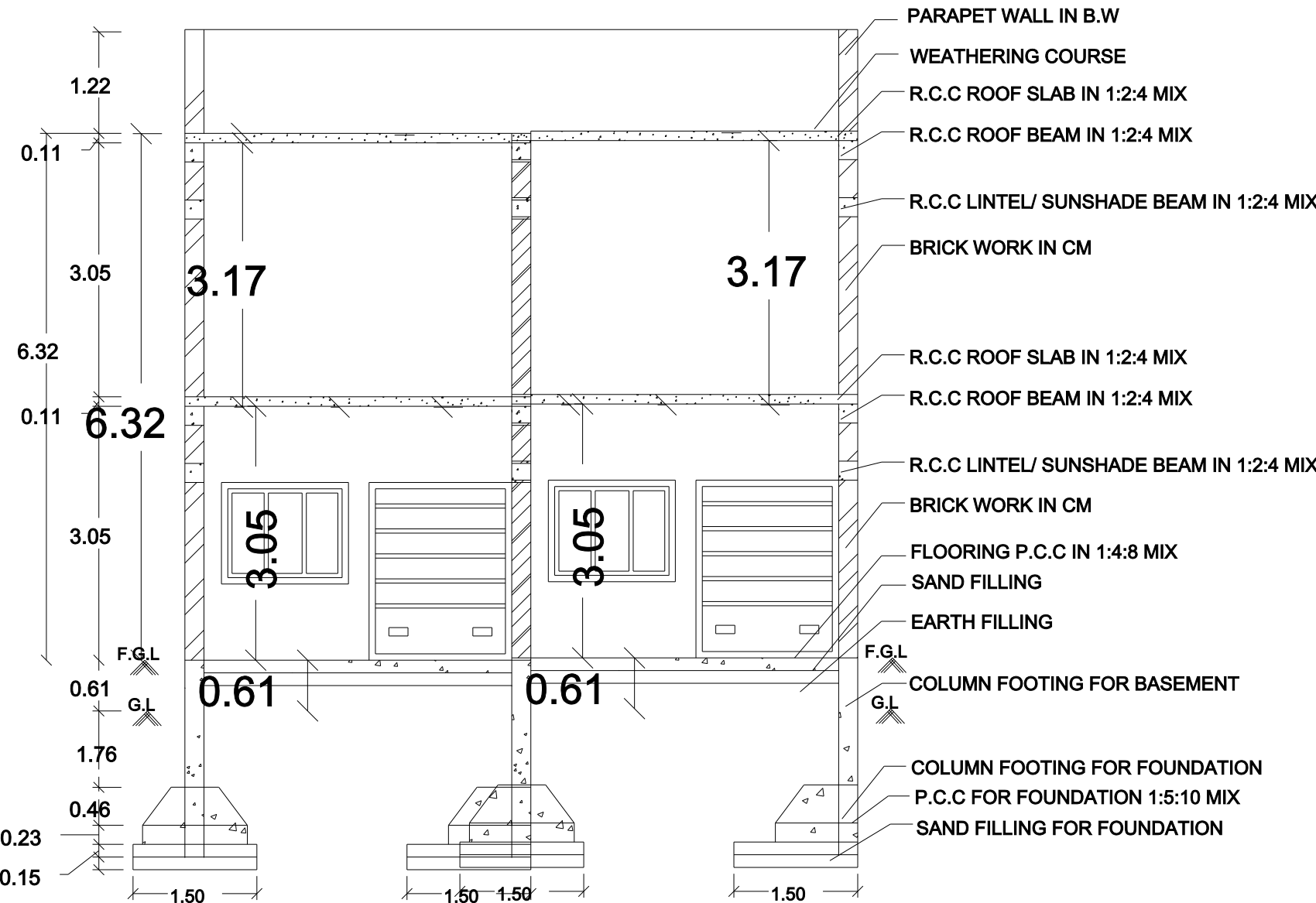
SECTION- BB
