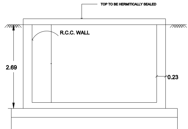
RWH_CAPACITY_L=5000LTRS
