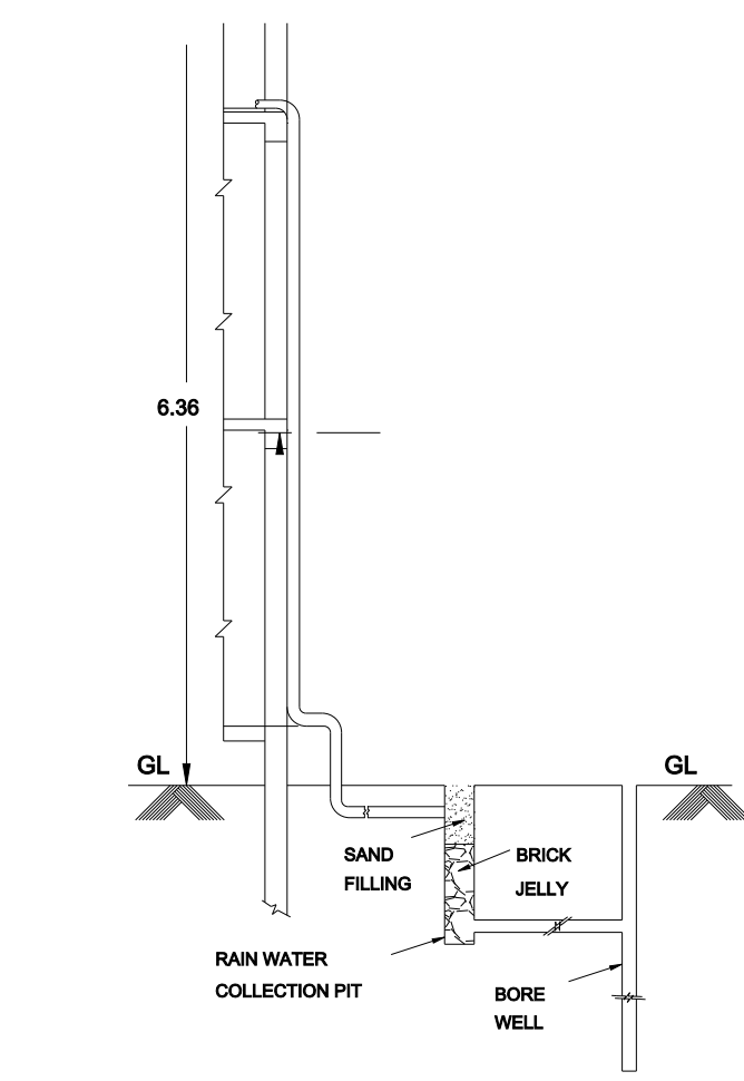
RAIN WATER HARVESTING SYSTEM
