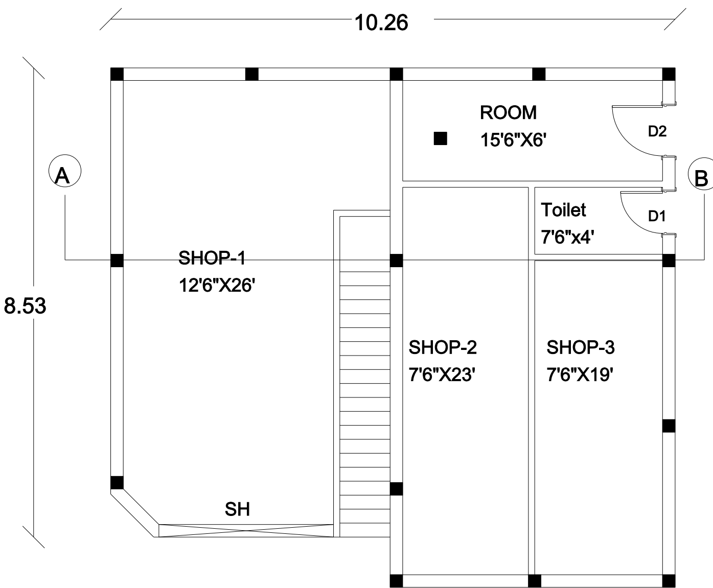
EX&PROPOSED GROUND FLOOR
