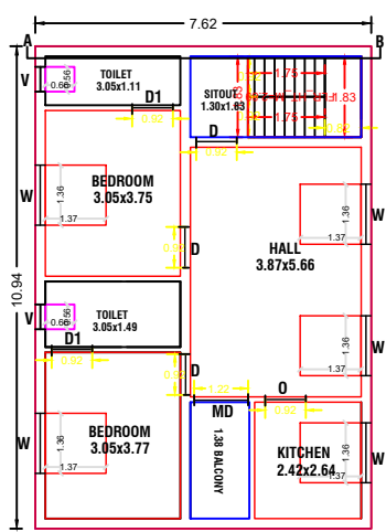
PRO., FIRST FLOOR PLAN
