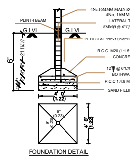
FOUNDATION DETAIL
