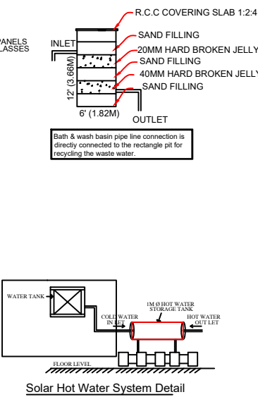
Solar Hot Water System Detail
