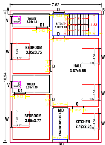
PRO., GROUND FLOOR PLAN
