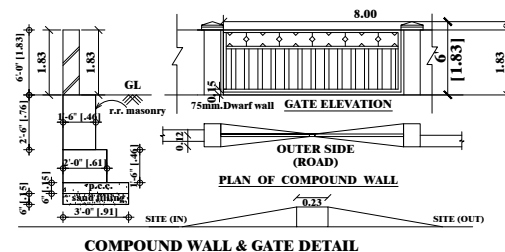
COMPOUND WALL & GATE DETAIL
