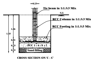
COLOUMN FOUNDATION DETAILS
