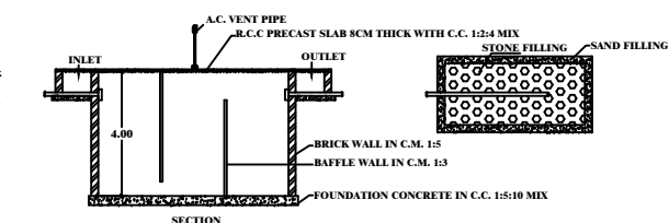
PLAN & SECTION OF SEPTIC TANK & DISPERSION TRENCH
