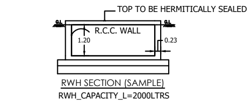
RWH SECTION (SAMPLE) RWH_CAPACITY_L=2000LTRS
