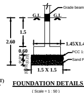
FOUNDATION DETAILS
