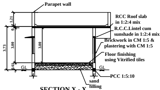
SECTION X - X
