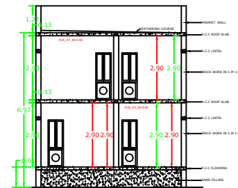
SECTION ON K-S
