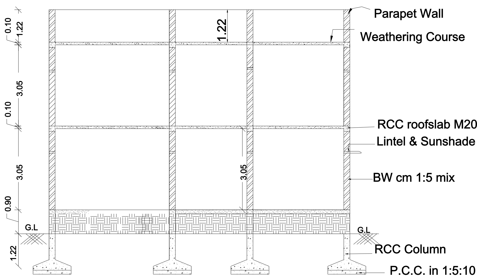
SECTION- BB
