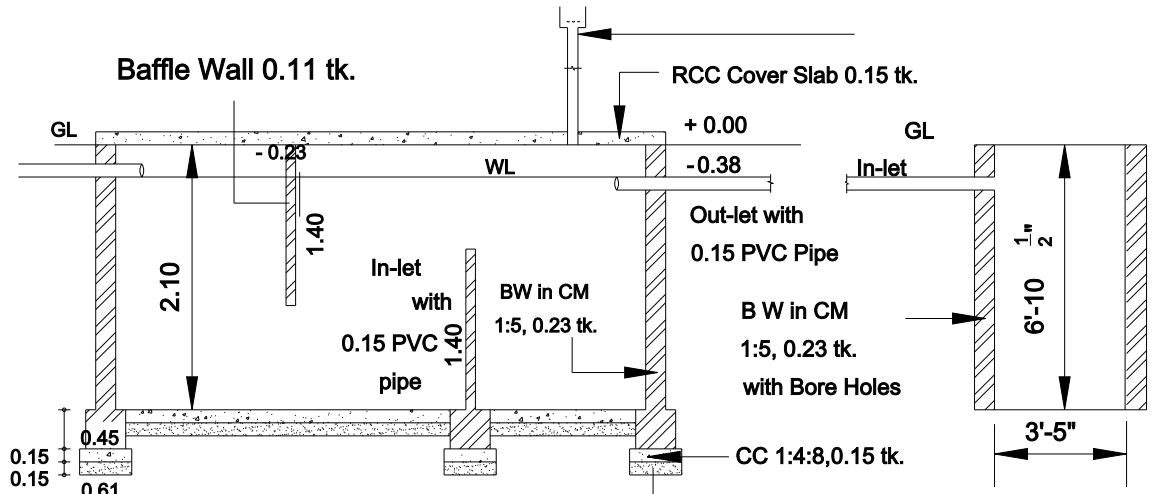
SECTION - SEPTIC TANK & SOAK PIT
