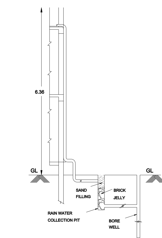
RAIN WATER HARVESTING SYSTEM RWH_CAPACITY_L=1000LTRS
