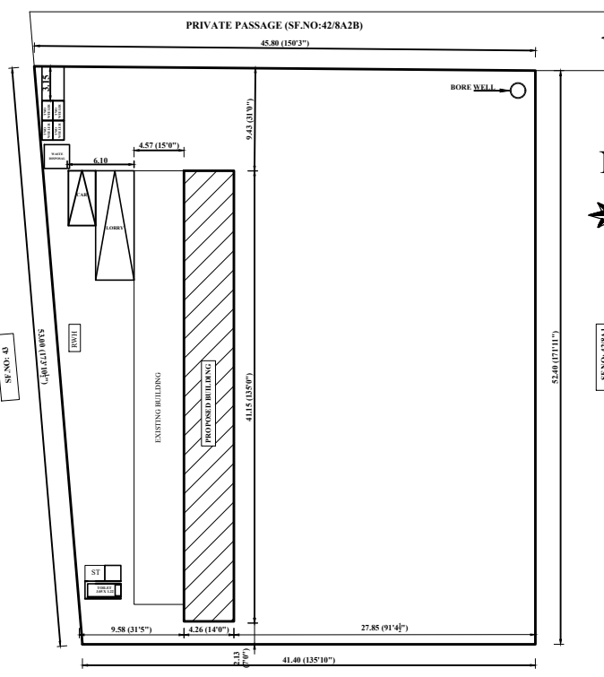
ROOF AREA PLAN
