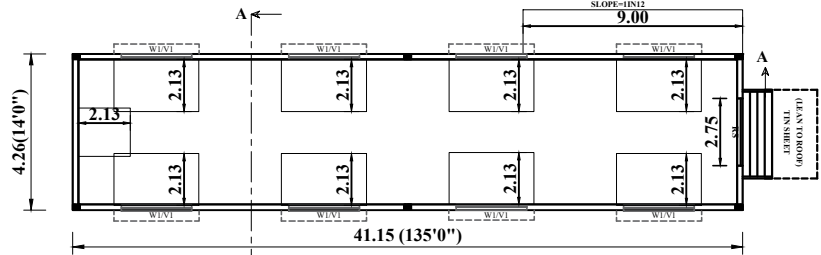
PROPOSED BUILDING PLAN
