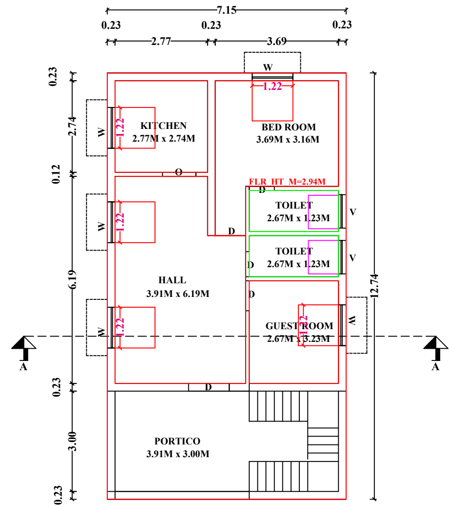
FLOOR-0
