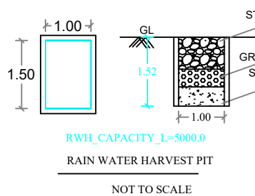
RAIN WATER HARVEST PIT NOT TO SCALE
