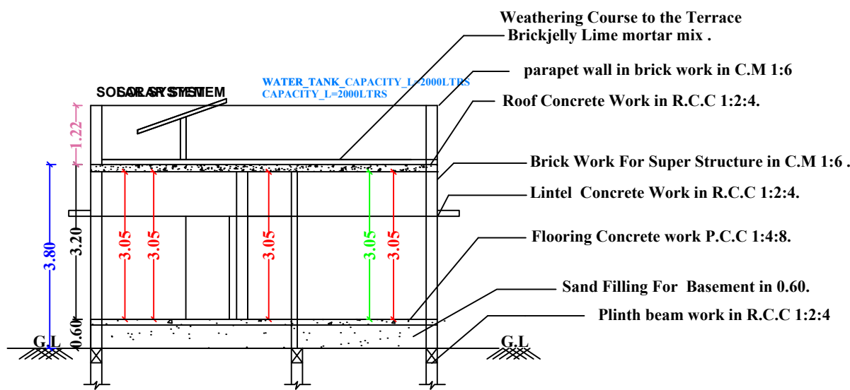
SECTION-AB
