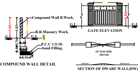
SECTION OF DWARF WALL(DW)
