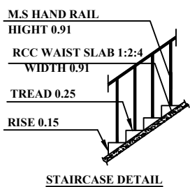
STAIRCASE DETAIL
