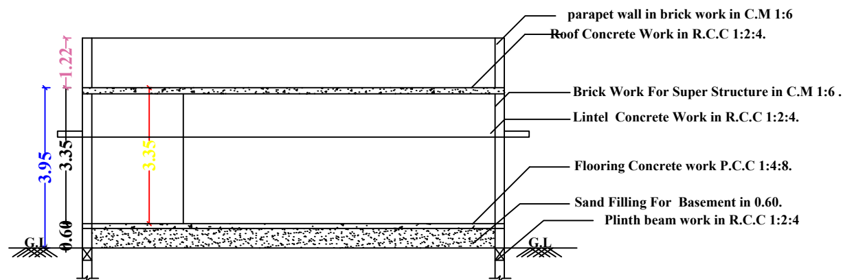
SECTION-AB
