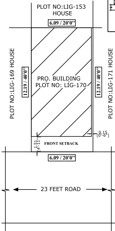
SITE PLAN
