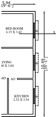
T FLOOR PLAN
