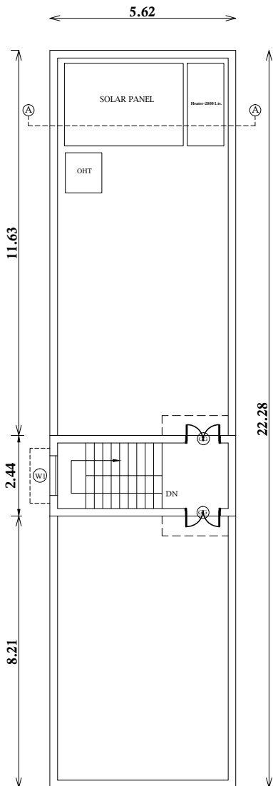
PRO FIRST FLOOR ROOF
