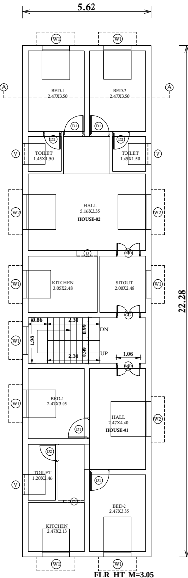
PRO FIRST FLOOR PLAN
