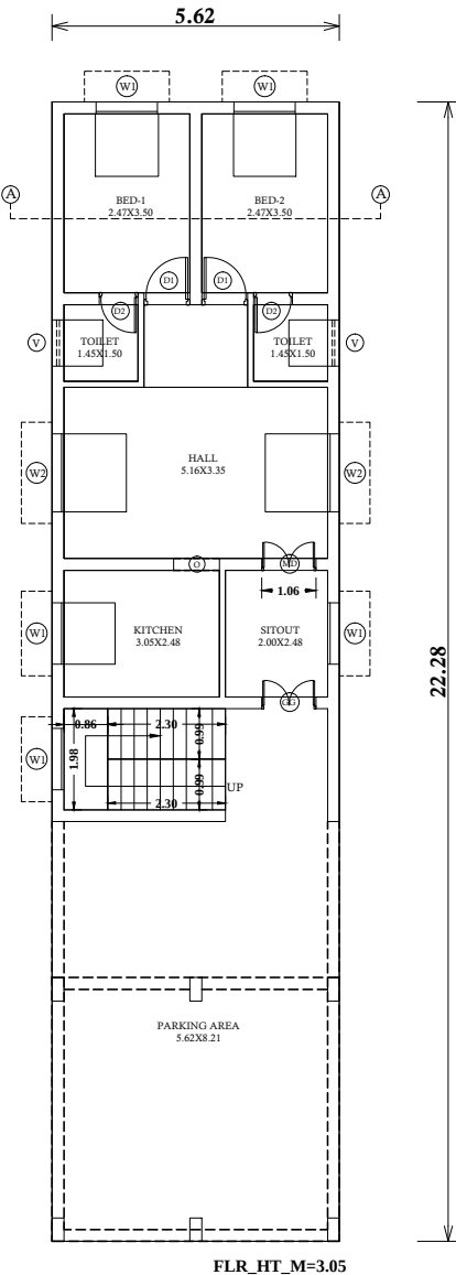
PRO GROUND FLOOR PLAN
