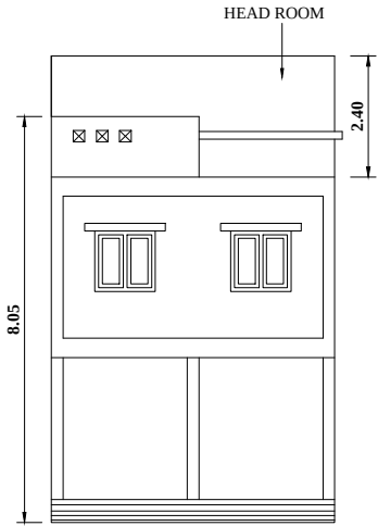
FRONT ELEVATION
