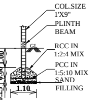
COLUMN DETAILS
