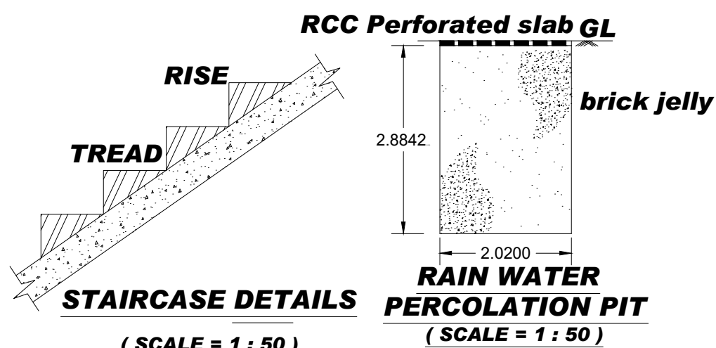
STAIRCASE DETAILS
