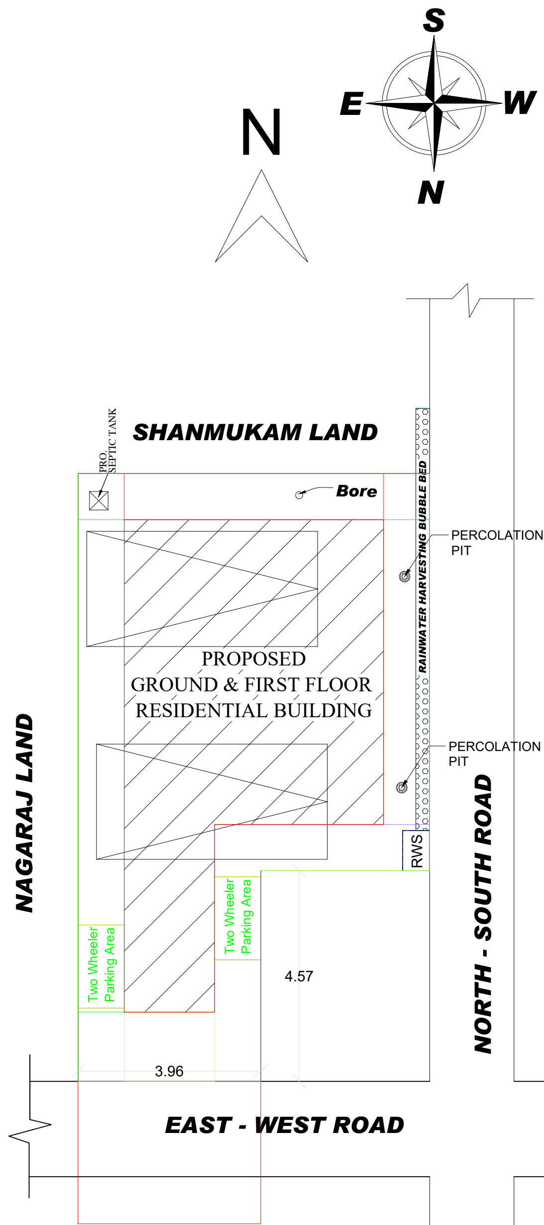
SITE PLAN (SCALE 1:1)
