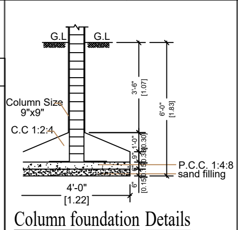
Column foundation Details
