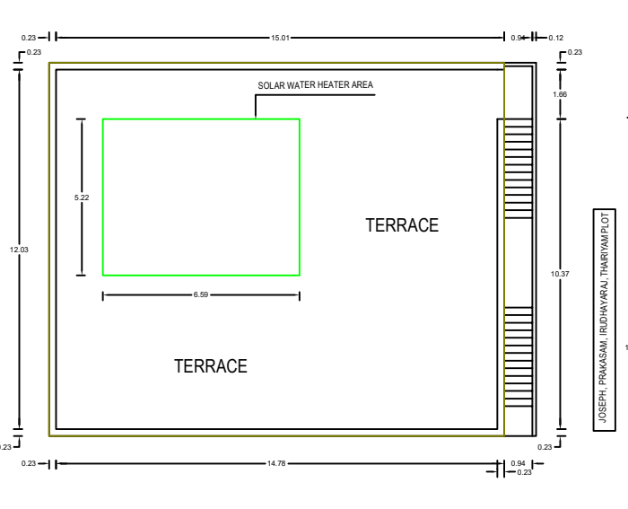
PRO. TERRACE FLOOR PLAN.
