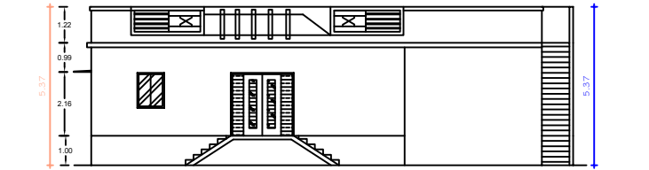
FRONT ELEVATION
