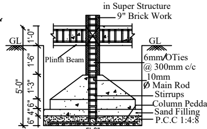
FOUNDATION DETAIL
