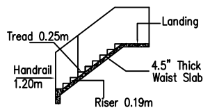
STAIRCASE DETAIL
