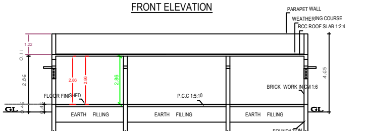
SECTION "A-B"
