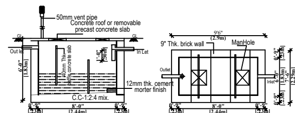
SECTION PLAN OF SEPTIC TANK
