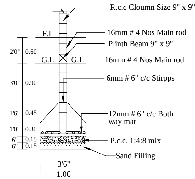
COLUMN DETIALS
