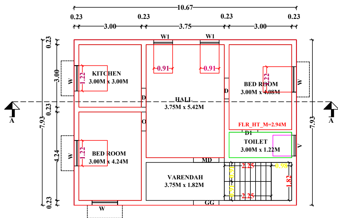
FLOOR-0 PRO.GROUND FLOOR PLAN
