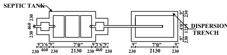
SEPTIC TANK DETAILS.
