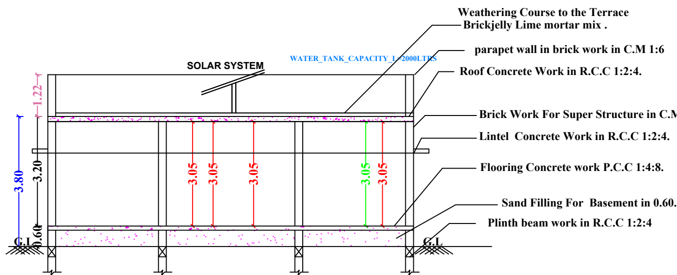
SECTION-AB
