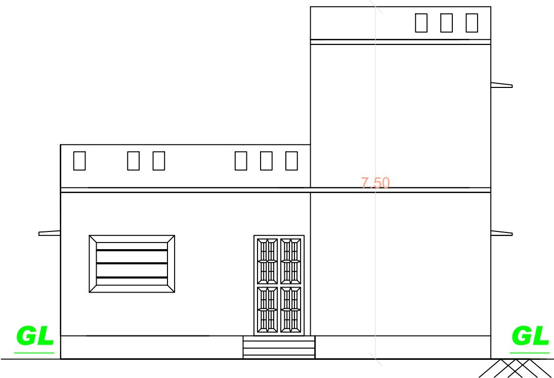
FRONT ELEVATION
