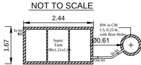
PLAN - SEPTIC TANK & SOAK PIT
