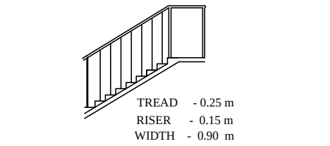
STAIRCASE DETAILS
