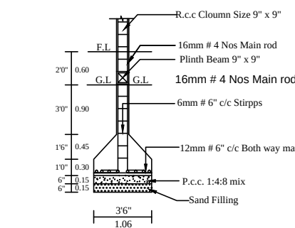
COLUMN DETIAL
