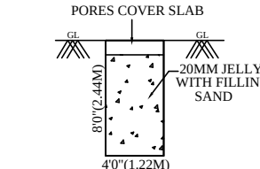
RAINWATER HARVESTING UNIT
