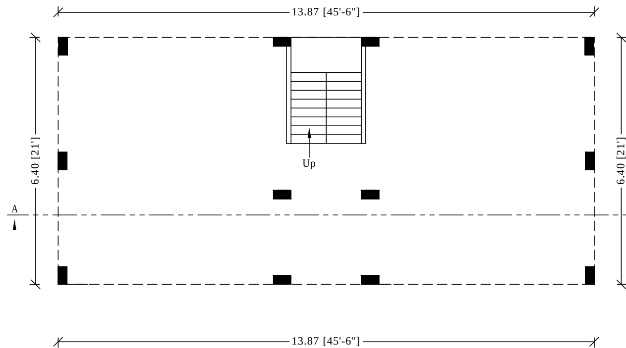
STILT FLOOR PLAN
