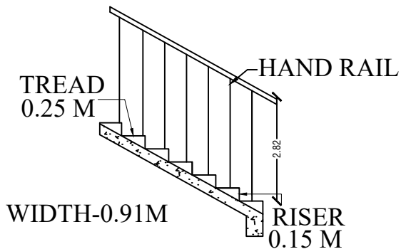
STAIRCASE DETAILS
