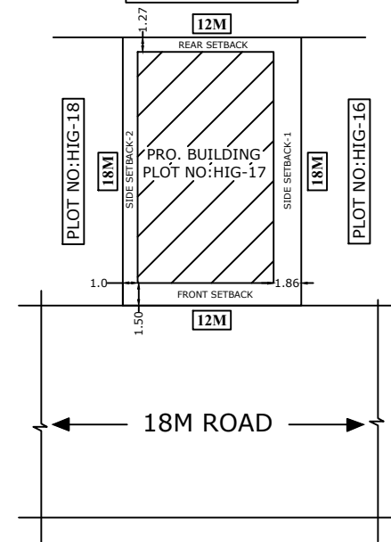
SITE PLAN
