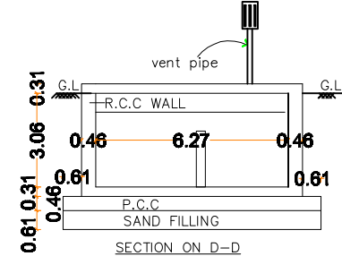
RWH SECTION (SAMPLE) RWH_CAPACITY_L = 2000.LTR
