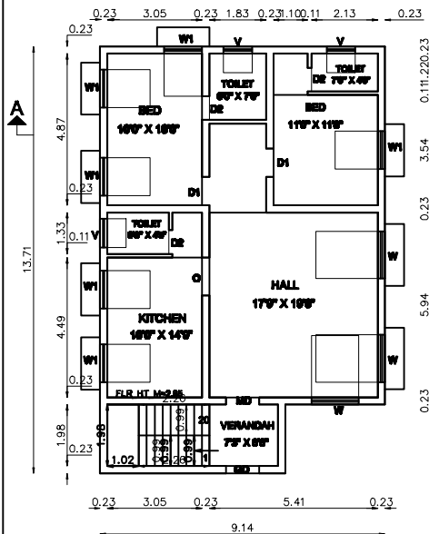
PRO.GROUND FLOOR PLAN SCALE: 1:100
