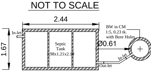
PLAN - SEPTIC TANK & SOAK PIT
