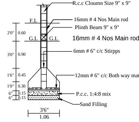
COLUMN DETIAL
