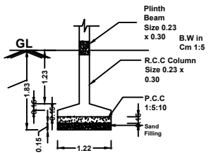
FOUNDATION DETAILS
