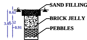
RAIN WATER HARVESTING SYSTEM
