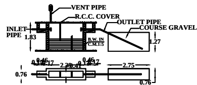
SEPTIC TANK & OF DISPERSION TRENCH DETAILS (NOT TO SCALE)
