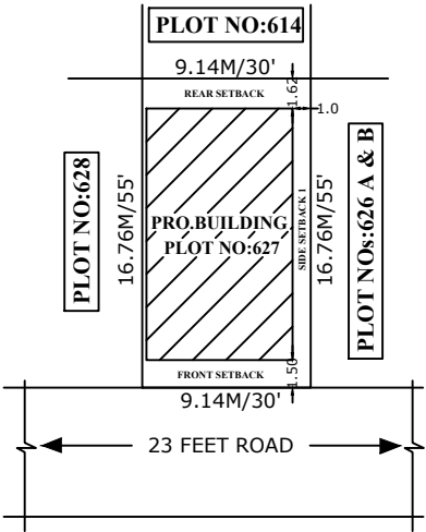
SITE PLAN
