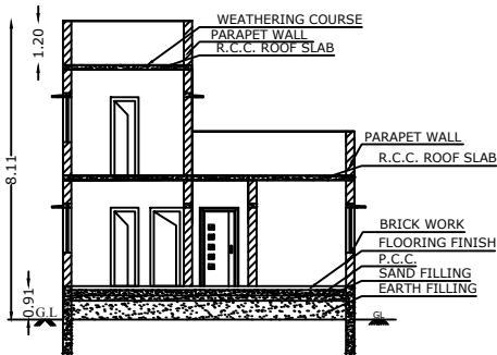
SECTION ON XX
