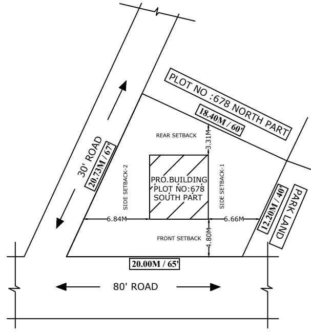
SITE PLAN
