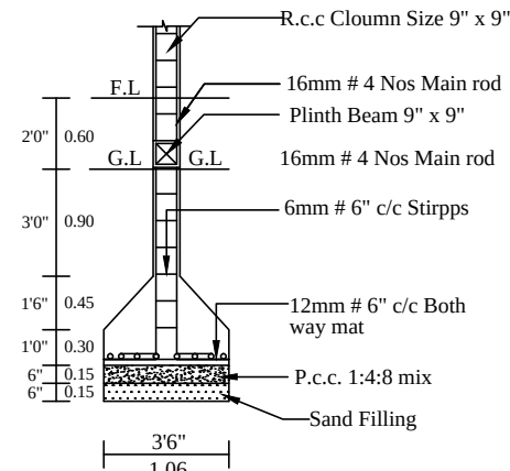
COLUMN DETIALS
