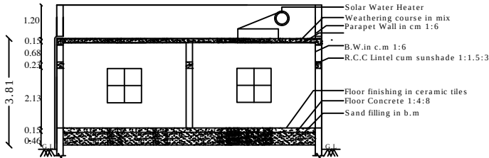
SECTION - "AB "
