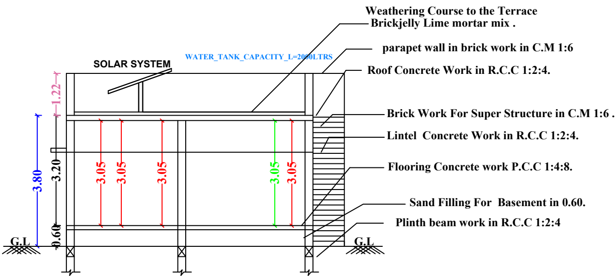
SECTION-AB
