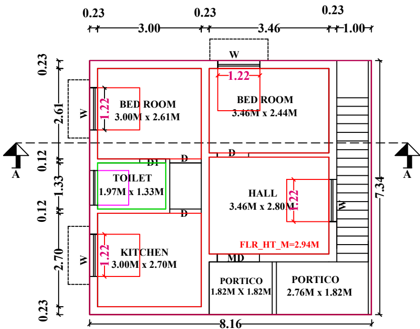
FLOOR-0 PRO.GROUND FLOOR PLAN
