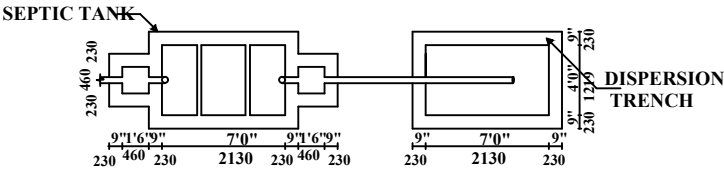
SEPTIC TANK DETAILS.
