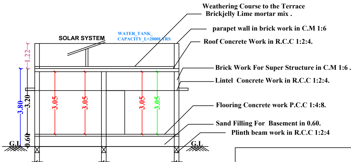
SECTION-AB
