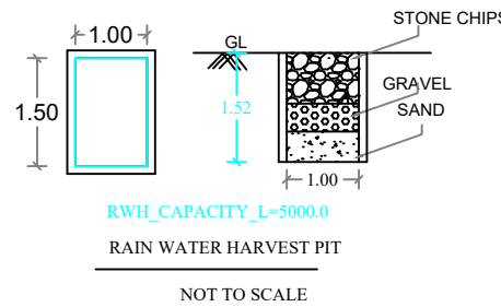
RAIN WATER HARVEST PIT
