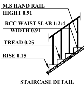
STAIRCASE DETAIL
