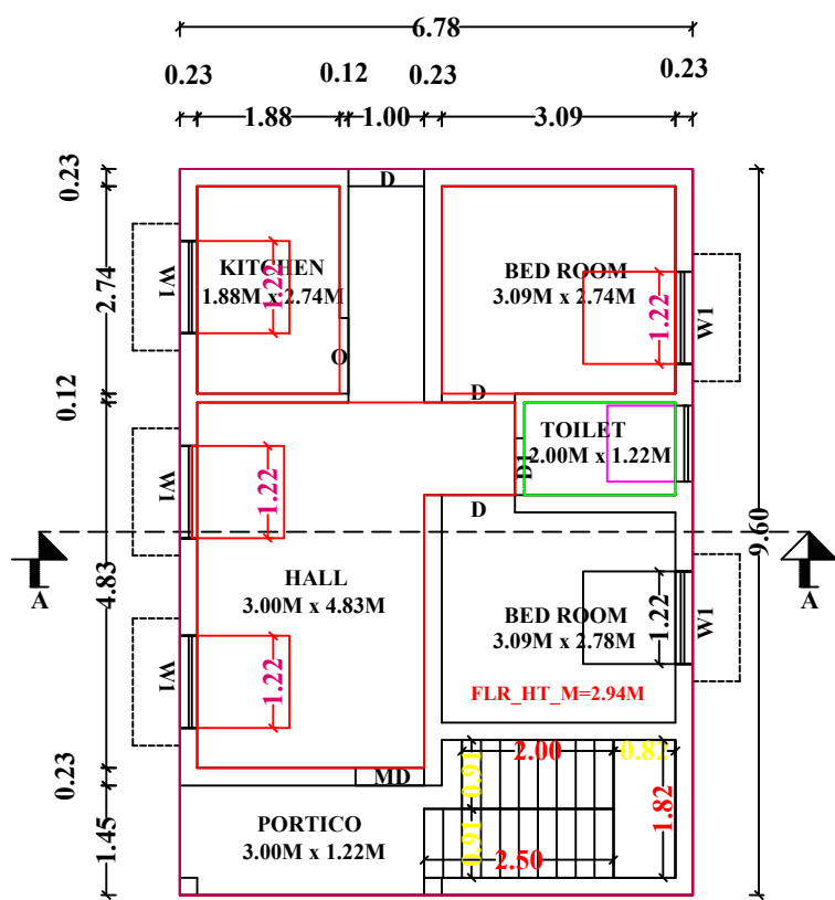
FLOOR-0
