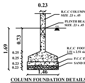
COLUMN FOUNDATION DETAILS
