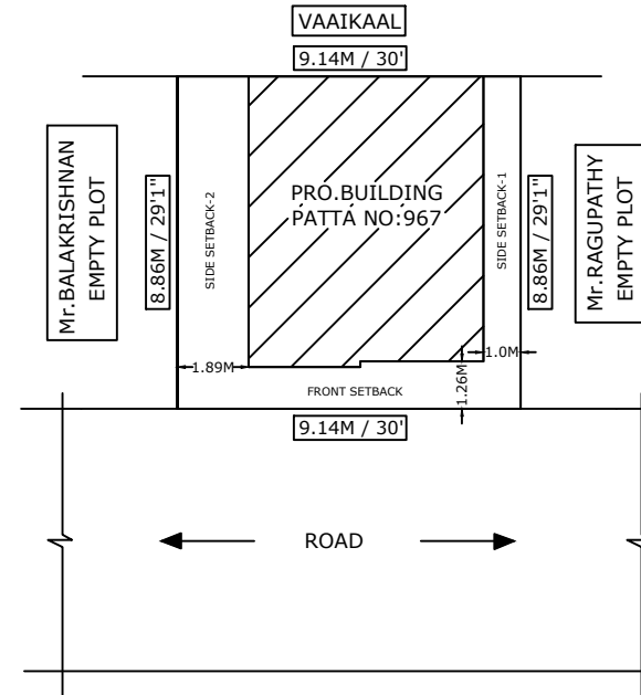
SITE PLAN
