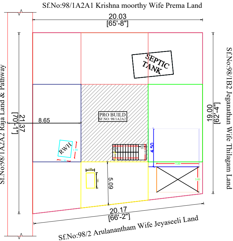
SITE PLAN (Not For Scale)
