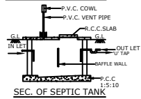
SEC. OF SEPTIC TANK
