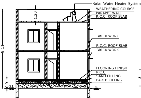
SECTION ON XX
