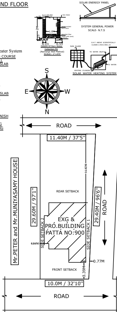
SITE PLAN
