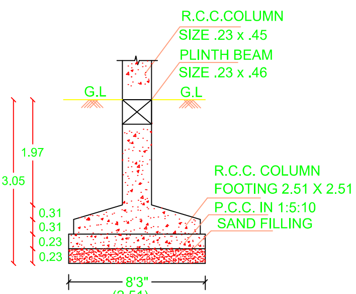
FOUNDATION DETAIL (DETAIL - B)
