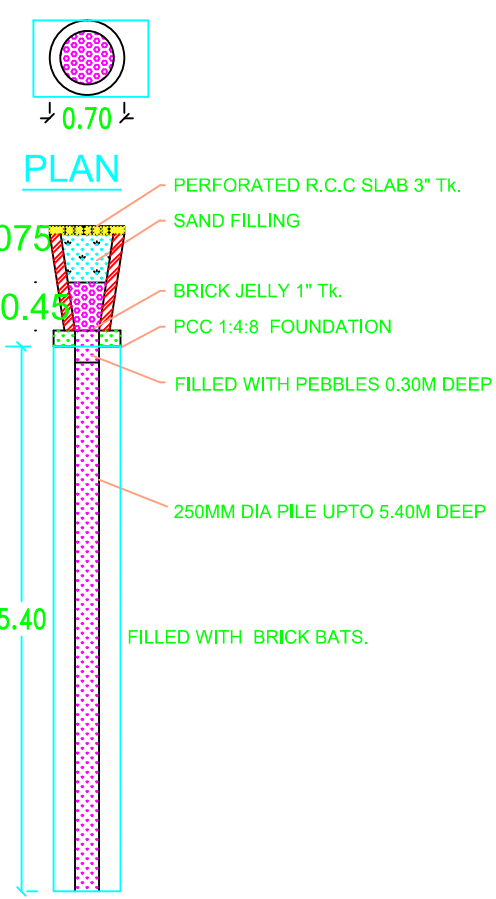
SECTION OF RAIN WATER RW_CAPACITY_1=500 (NOT TO SCALE)
