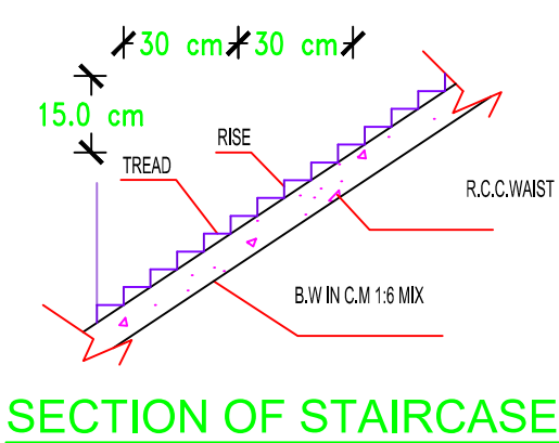
SECTION OF STAIRCASE
