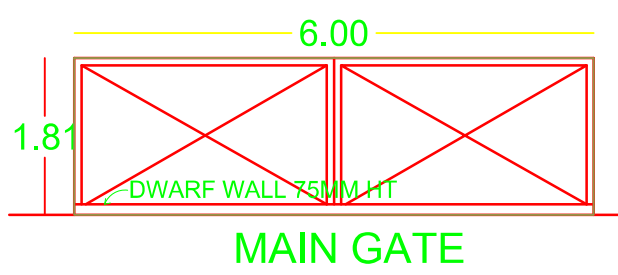
MAIN GATE
