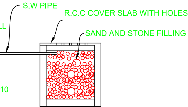
DETAILS OF DISPERSION TRENCH (NOT TO SCALE)
