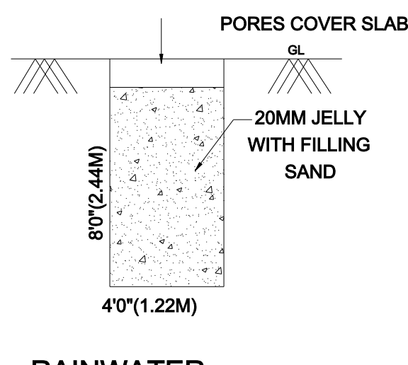
RAINWATER HARVESTING UNIT
