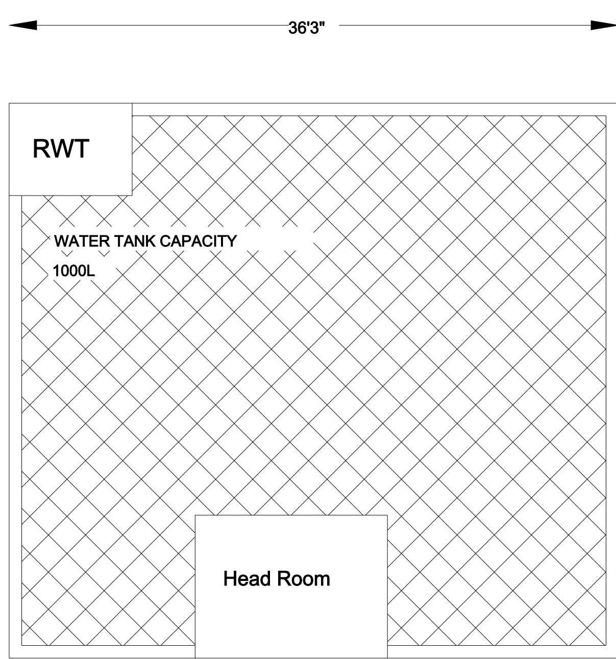
ROOF PLAN
