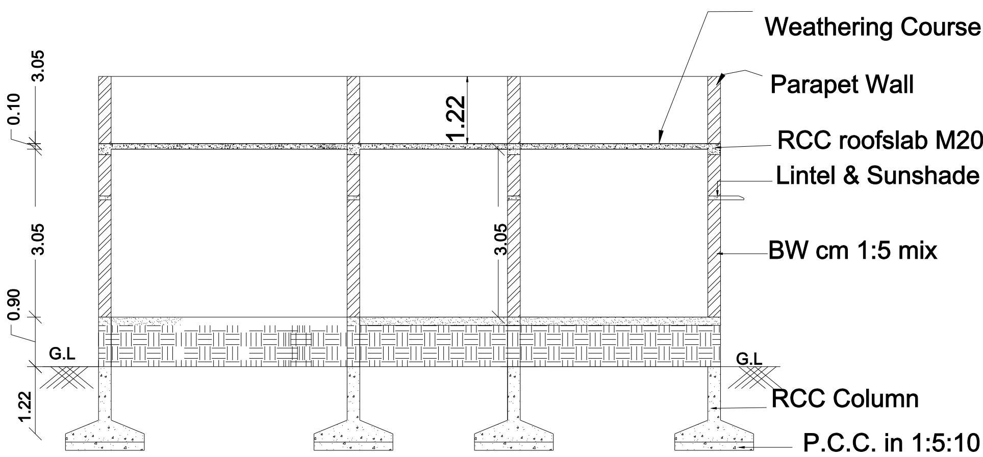
SECTION- BB
