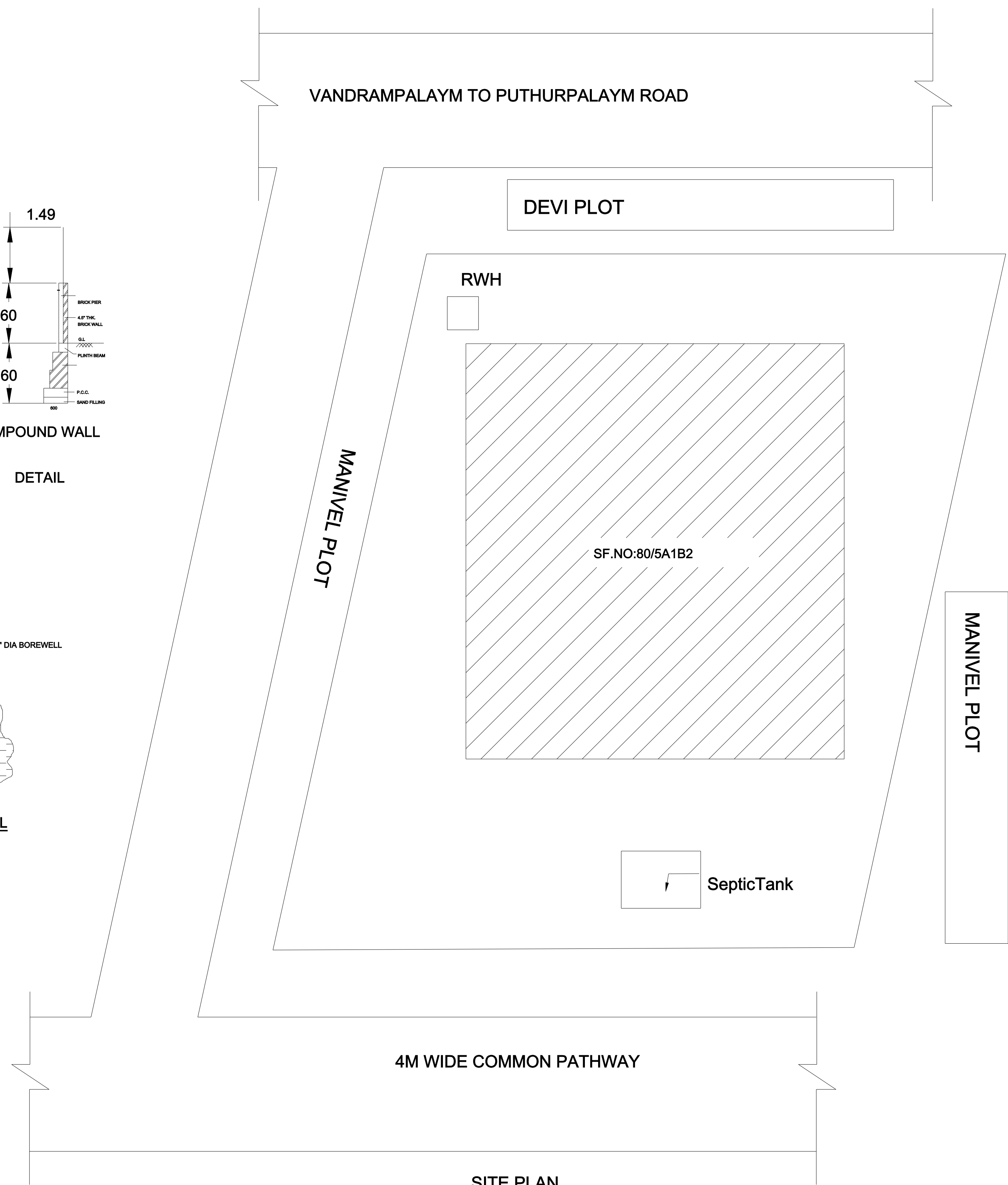
SITE PLAN
