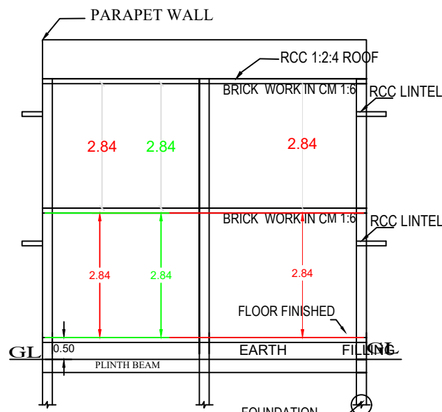
SECTION "A-B".
