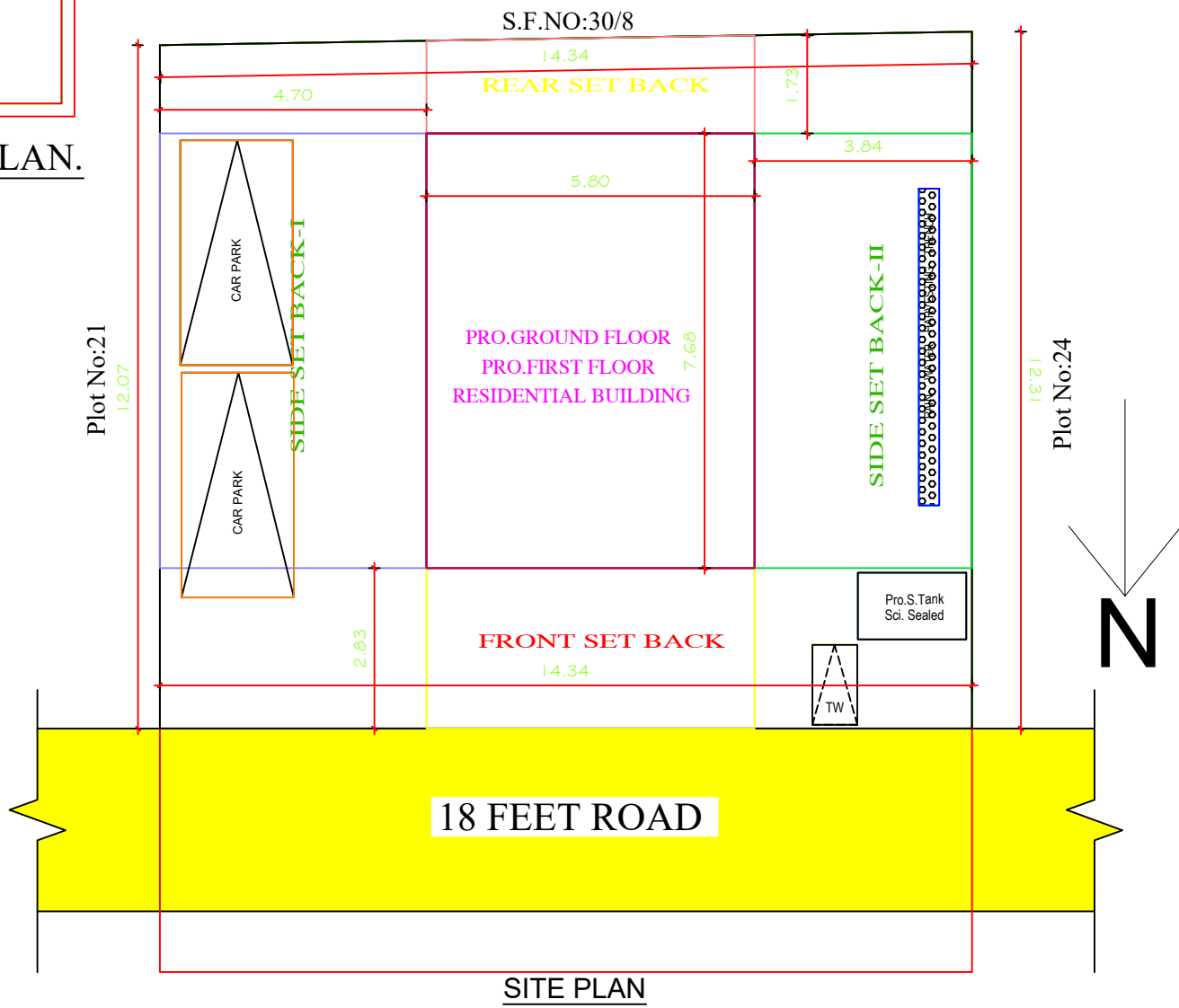
SITE PLAN
