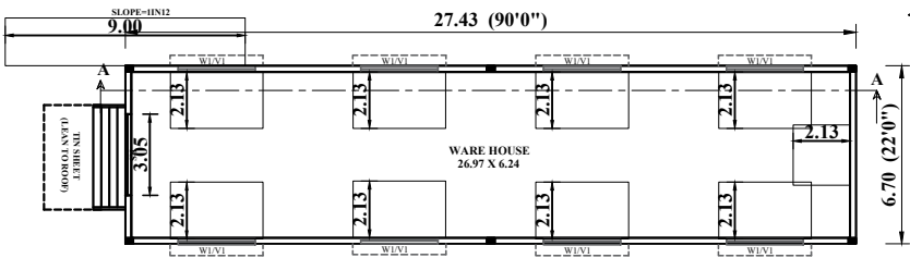
PROPOSED BUILDING PLAN
