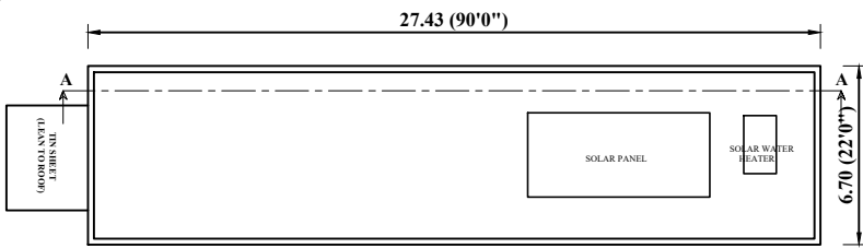
ROOF AREA PLAN
