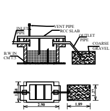
SEPTIC TANK & D-TRENCH DETAILS (NOT TO SCALE)
