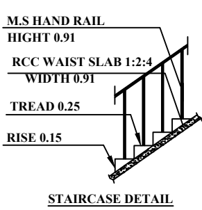
STAIRCASE DETAIL
