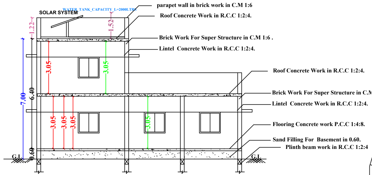
SECTION-AB
