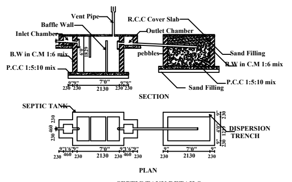
SEPTIC TANK DETAIL
