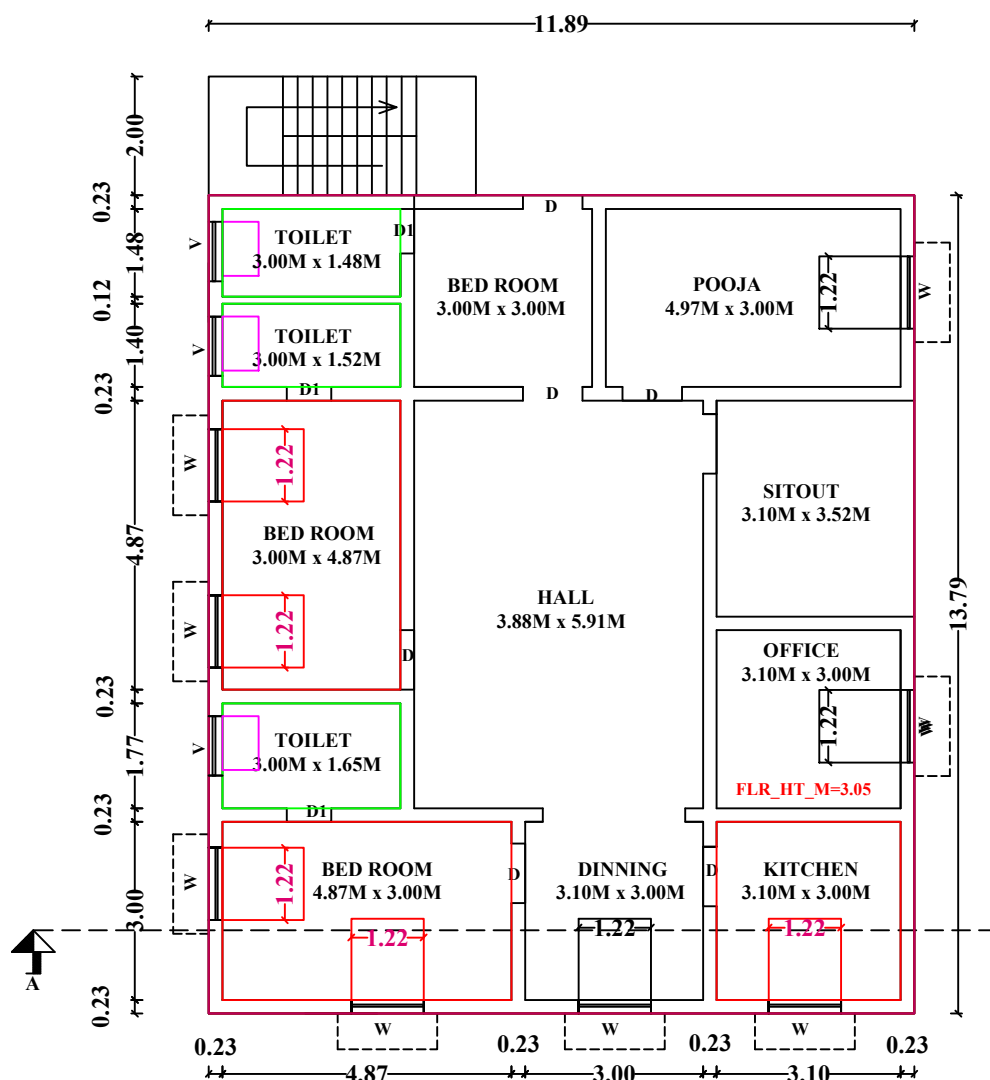
FLOOR-0 PRO.GROUND FLOOR PLAN
