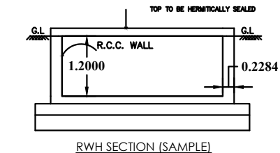
RWH_CAPACITY_L=2000LTRS
