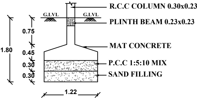
COLUMN FOUNDATION (NOT TO SCALE)
