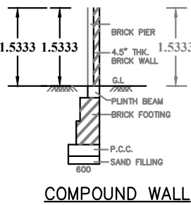
COMPOUND WALL
