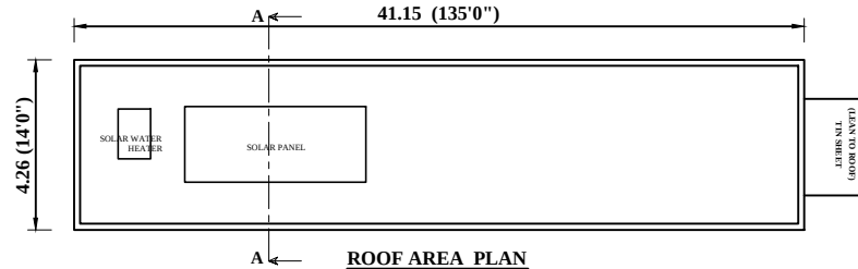
ROOF AREA PLAN
