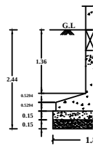
COLUMN FOUNDATION (DE)
